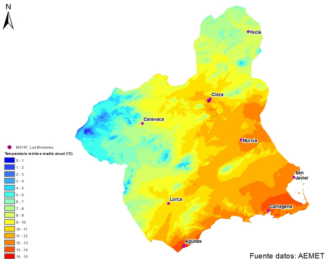
FIGURA 6. T^a min anual ( ^{\circ}\text{C} )
